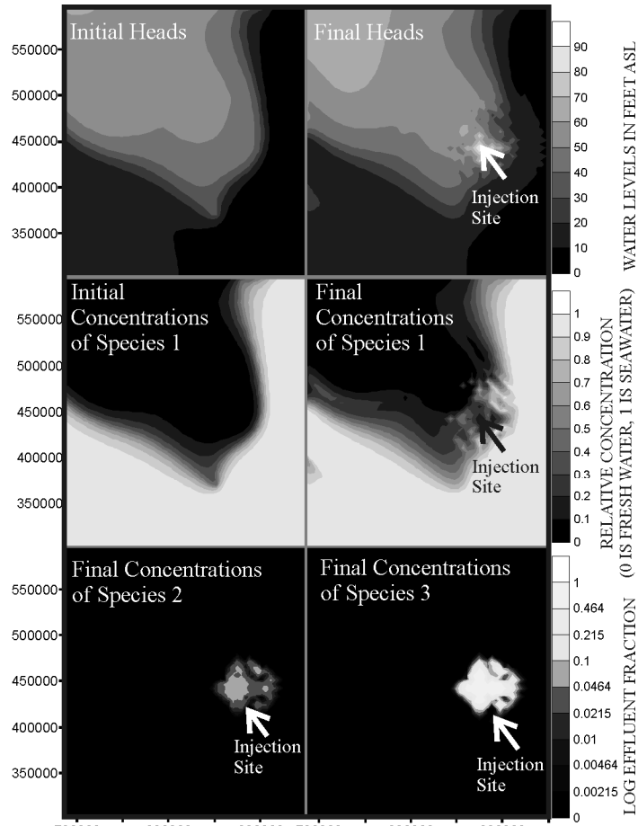
Figure 3: Map view of the MFA showing initial heads and concentrations, and final heads and concentrations of species 1, 2, and 3 after 148 years of injection. Coordinates are in feet, State Plane 83.
